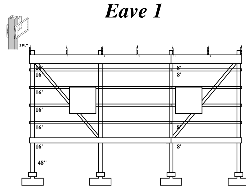
SAMPLE WALL SECTION
