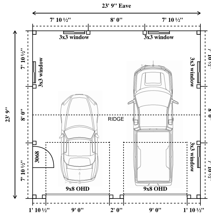
POST PLAN
