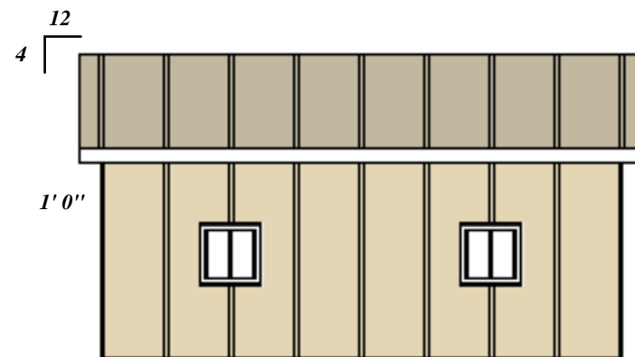
EAVE 1
